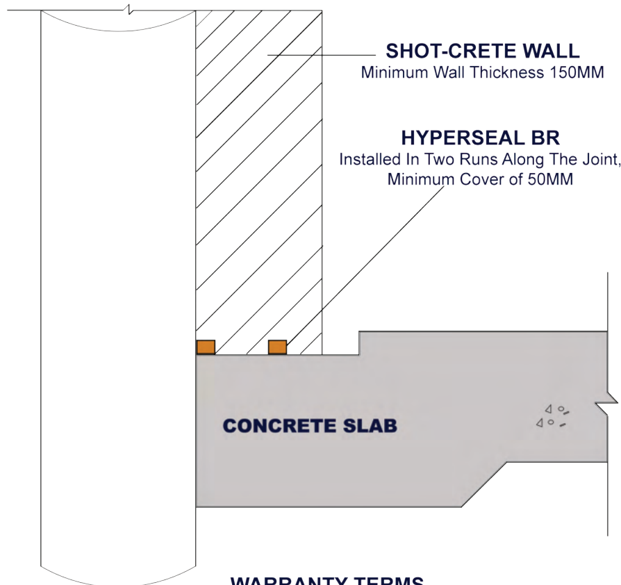
CROSS SECTION
